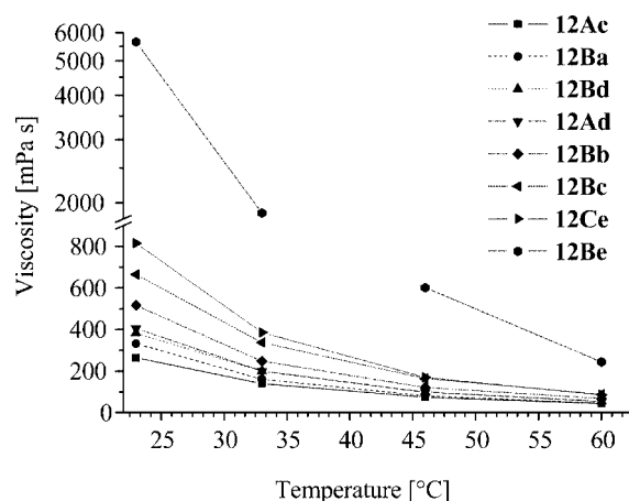
Figure 2. Viscosity of some salts 12 as a function of temperature.
