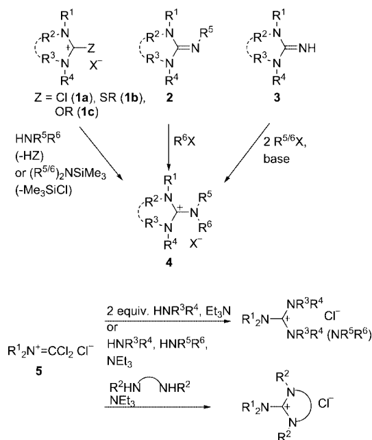
Scheme 1. Synthetic pathways to hexaalkylguanidinium salts.
