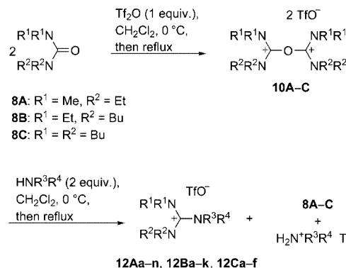
Scheme 4. Synthesis of guanidinium triflates 12 .
