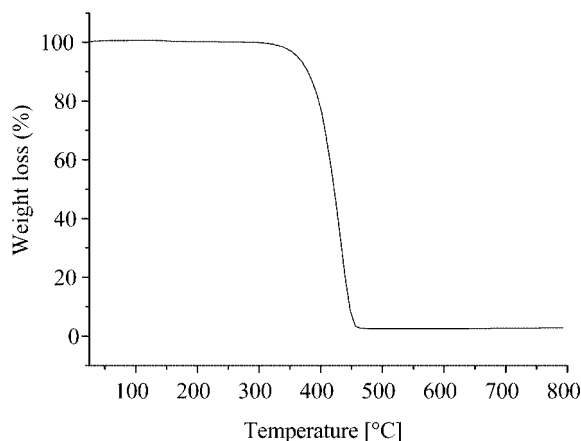
Figure 1. TGA curve for salt 12Bc .
