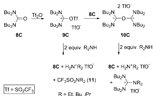
Scheme 3. Reaction of uronium salts 9C and 10C with sec -amines.
