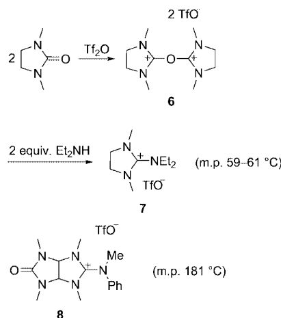
Scheme 2. Cyclic hexasubstituted guanidinium triflates 7 and 8 .
